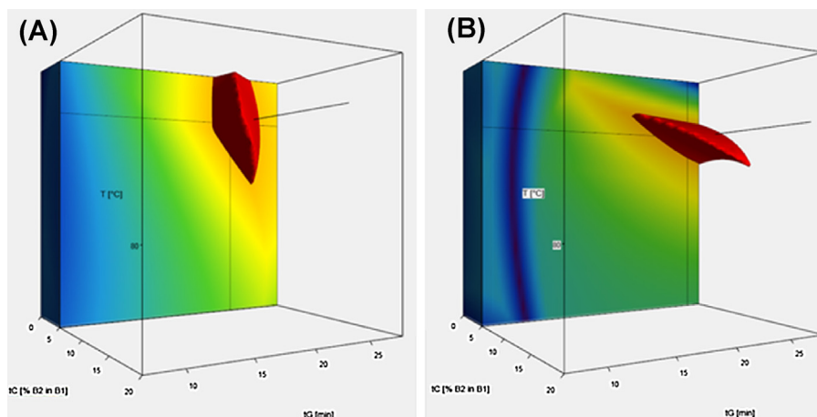
Fig. 6. 3D resolution maps for Brentuximab vadotin (A) and for Brentuximab vedotin reduced (B) samples, based on the initial experiments ( R_s crit = 1.0). Set conditions for the native sample: t_G = 23 min, T = 88 °C and t_C = 5% MeOH. Set conditions for the reduced sample: t_G = 27 min, T = 87 °C and t_C = 5% MeOH. (For interpretation of the references to colour in the text, the reader is referred to the web version of this article.)
