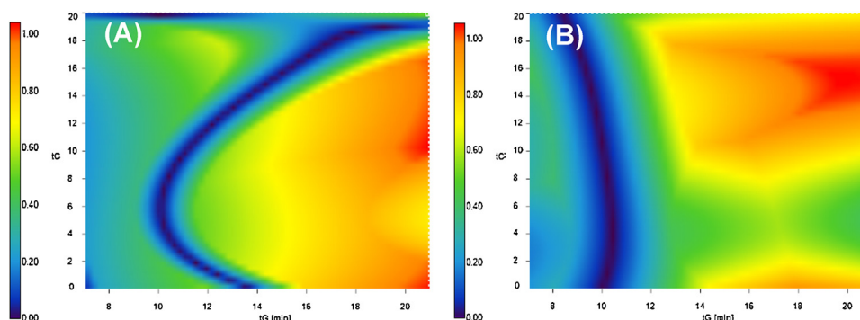
Fig. 12. Simplified 2D resolution maps of native (A) and reduced (B) ADC based on six initial experiments ( t_G \times t_C model). Gradient: 25–50% B, t_{G1} = 10 min, t_{G2} = 20 min, t_{C1} = 0\% MeOH, t_{C2} = 10\% MeOH and t_{C3} = 20\% MeOH, T = 90^\circ\text{C} . (Column: Agilent Advance BioMAb RP C4, flow rate: 0.3 mL/min).
