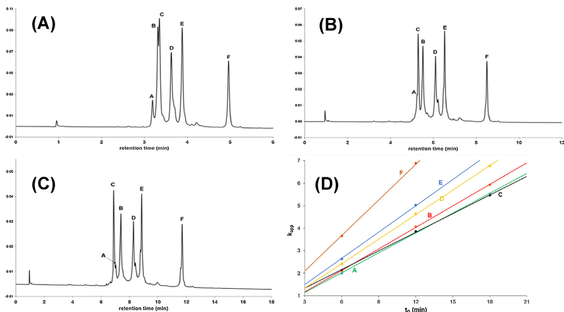
Fig. 1. The impact of gradient steepness on selectivity. Column: Agilent Advance BioMab RP C4. Mobile phase “A”: 0.1% TFA in water, “B”: 0.1% TFA in acetonitrile. Flow rate: 0.3 mL/min, gradient: 25–50% B (in 6 min (A), 12 min (B) and 18 min (C)), temperature: 90 °C, injected volume: 1 \mu L, detection at 280 nm. Panel D shows the dependence of k_{app} on the gradient time. Sample: Brentuximab vedotin.
