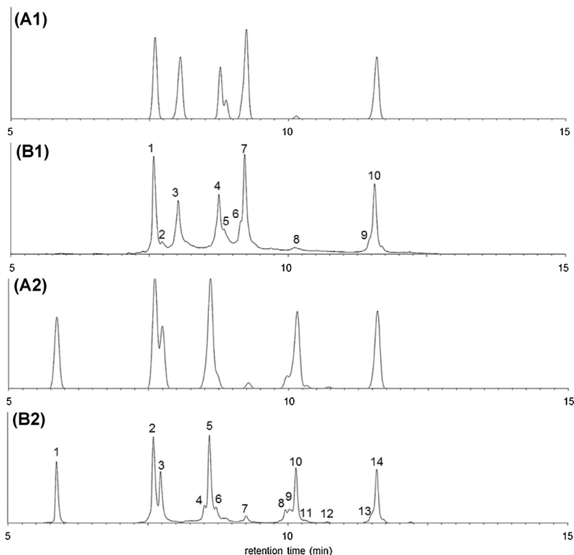
Fig. 5. Model verification in the center point for native Brentuximab vedotin (1) and for reduced Brentuximab vedotin (2). Column: Agilent Advance BioMAb RP C4. Mobile phase “A”: 0.1% TFA in water, “B”: 0.1% TFA in 90% acetonitrile + 10% MeOH. Flow rate: 0.3 mL/min, gradient: 25–50% B in 15 min, temperature: 82.5 °C, injected volume: 1 \mu L, detection at 280 nm. “A” corresponds to predicted, while “B” corresponds to experimental chromatograms.
