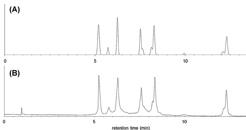
Fig. 7. Predicted (A) and experimentally verified (B) chromatograms of native Brentuximab vedotin under optimal conditions. Gradient: 29–42% B, t_G = 14 min, T = 90 °C and t_C = 0% MeOH (100% AcN). (Column: Agilent Advance BioMab RP C4, flow rate: 0.3 mL/min).
