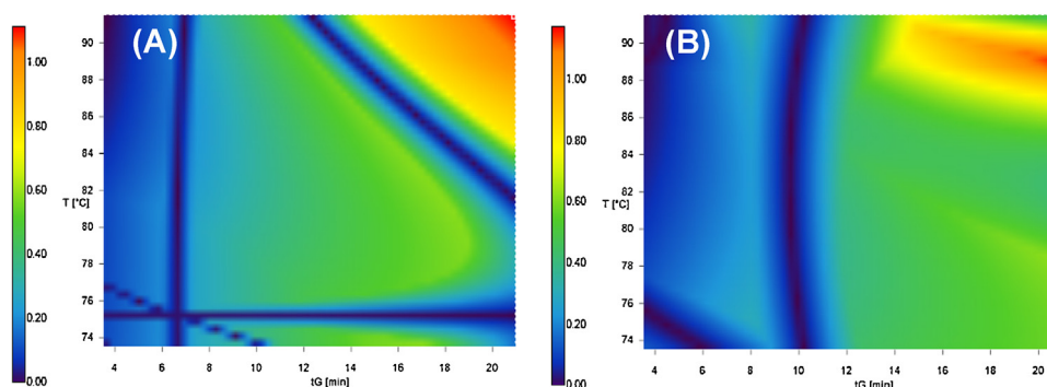
Fig. 11. Simplified 2D resolution maps of native (A) and reduced (B) ADC based on four initial experiments ( t_G \times T model). Gradient: 25–50% B, t_{G1} = 10 min, t_{G2} = 20 min, T_1 = 75^\circ\text{C} , T_2 = 90^\circ\text{C} and t_C = 0\% MeOH (100% AcN). (Column: Agilent Advance BioMab RP C4, flow rate: 0.3 mL/min).
