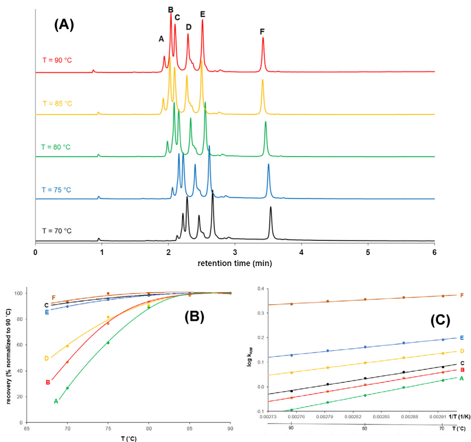
Fig. 2. The impact of mobile phase temperature on the retention times (A), peak area (recovery) (B) and retention factor (C) of different ADC species. Column: Agilent Advance BioMab RP C4. Mobile phase “A”: 0.1% TFA in water, “B”: 0.1% TFA in acetonitrile. Flow rate: 0.3 mL/min, gradient: 30–60% B in 6 min (extended gradient to enable baseline resolution and the measurement of peak areas), temperature: 90 °C, injected volume: 1 \mu L, detection at 280 nm. Sample: Brentuximab vedotin.
