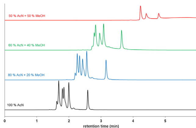
Fig. 3. The impact of mobile phase ternary composition. Column: Agilent Advance BioMab RP C4. Mobile phase "A": 0.1% TFA in water, "B": 0.1% TFA in acetonitrile and methanol mixture. Flow rate: 0.3 mL/min, gradient: 30–80% B in 6 min (extended gradient to enable eluting all the peaks with 50% MeOH content), temperature: 90^\circ\text{C} , injected volume: 1 \mu\text{L} , detection at 280 nm. Sample: Brentuximab vedotin.
