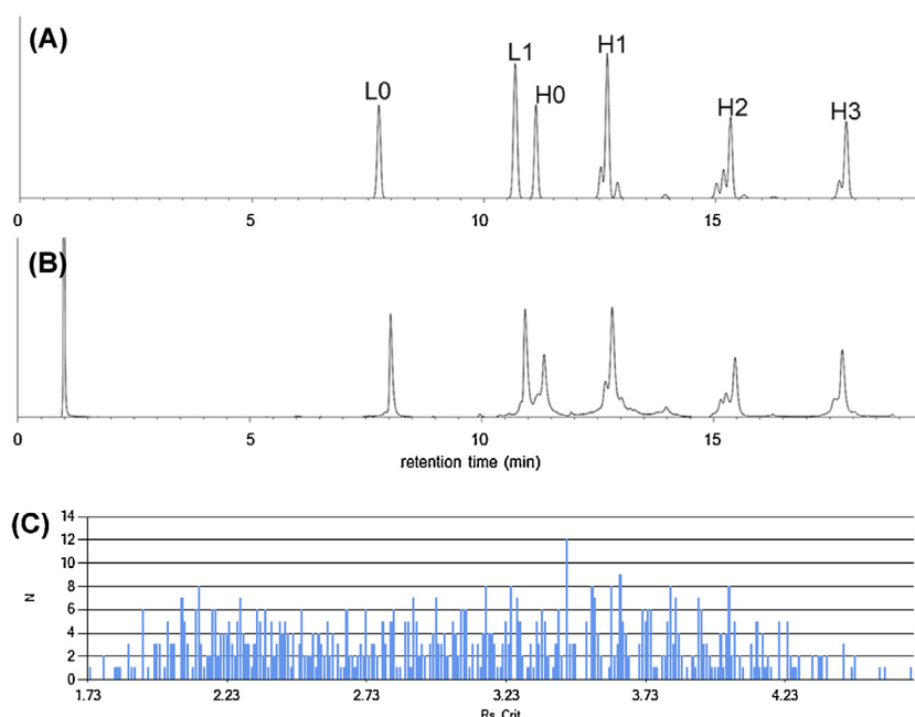
Fig. 9. Predicted (A) and experimentally verified (B) chromatograms of reduced Brentuximab vedotin under optimal conditions to optimize resolution between all peaks. Gradient: 25–50% B, t_G = 27 min, T = 87^\circ\text{C} and t_C = 5\% MeOH (95% AcN). (Column: Agilent Advance BioMab RP C4, flow rate: 0.3 mL/min). Panel C represents the result of simulated robustness test as number of observations (N) vs. critical resolution ( R_{s,\text{crit}} ).
