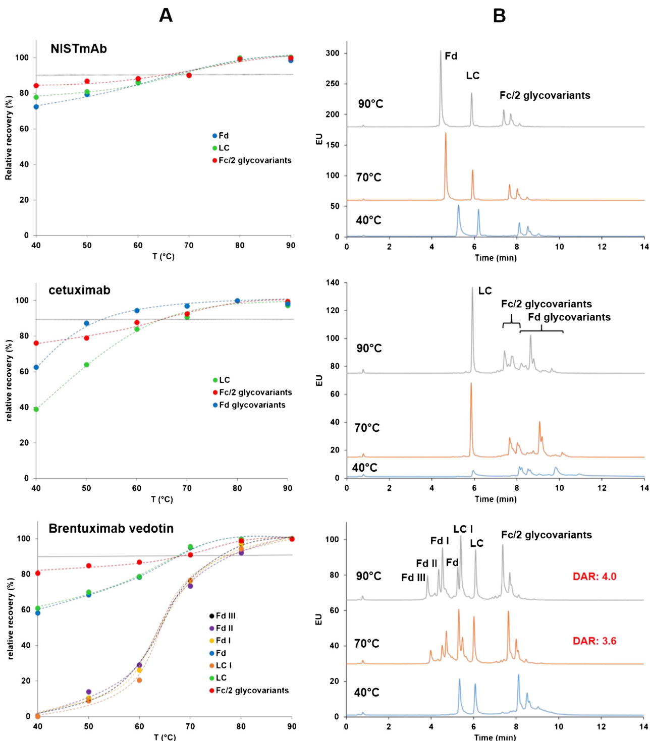
Fig. 3. (A) Relative recovery of NISTmAb, cetuximab and brentuximab vedotin subunits as a function of mobile phase temperature. (B) Corresponding chromatograms at 40 °C, 70 °C and 90 °C. Gradient: 75–60%B in 15 min. A: H 2 O + 0.1% TFA, B: ACN + 0.1% TFA. Flow: 0.45 mL/min. Column: Waters Acquity UPLC Glycoprotein BEH Amide (300 Å, 1.7 μm, 2.1 mm × 150 mm).
