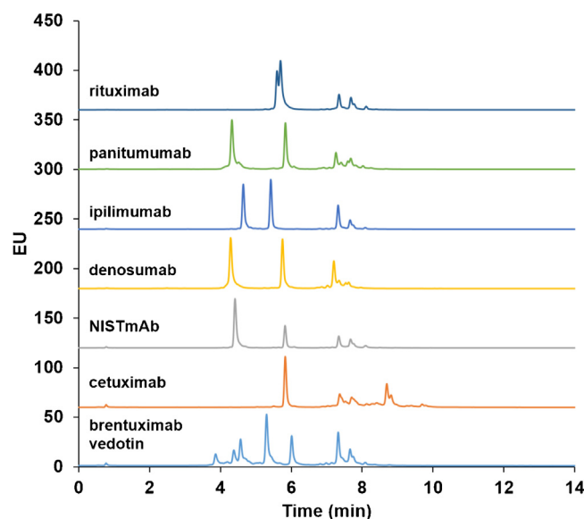
Fig. 2. General HILIC chromatograms of IdeS digested and reduced mAb and ADC samples. Gradient: 75–60%B in 15 min. A: H 2 O + 0.1% TFA, B ACN + 0.1% TFA. T: 80 °C, flow: 0.45 mL/min. Column: Waters Acquity UPLC Glycoprotein BEH Amide (300 Å, 1.7 μm, 2.1 mm × 150 mm).
