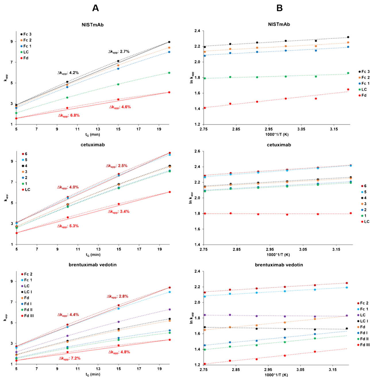
Fig. 4. (A) Retention as a function of gradient time, (B) Van't Hoff plots of NISTmAb, cetuximab and brentuximab vedotin subunits. Gradient: 75–60%B. A: H 2 O + 0.1% TFA, B: ACN + 0.1% TFA, flow: 0.45 mL/min. Column: Waters Acquity UPLC Glycoprotein BEH Amide (300 Å, 1.7 \mu m, 2.1 mm \times 150 mm). Other chromatographic conditions are detailed in Section 3.3.
