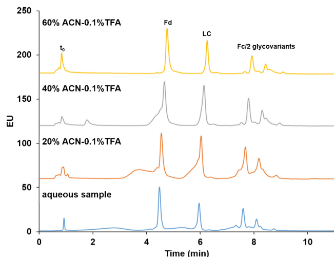
Fig. 1. HILIC chromatograms of IdeS digested and reduced trastuzumab when injecting from different sample solvents and using linear gradient without initial fast gradient ramp. Gradient: 74–68%B in 15 min. A: H 2 O + 0.1% TFA, B ACN + 0.1% TFA. Other chromatographic conditions are detailed in Section 2.3.
