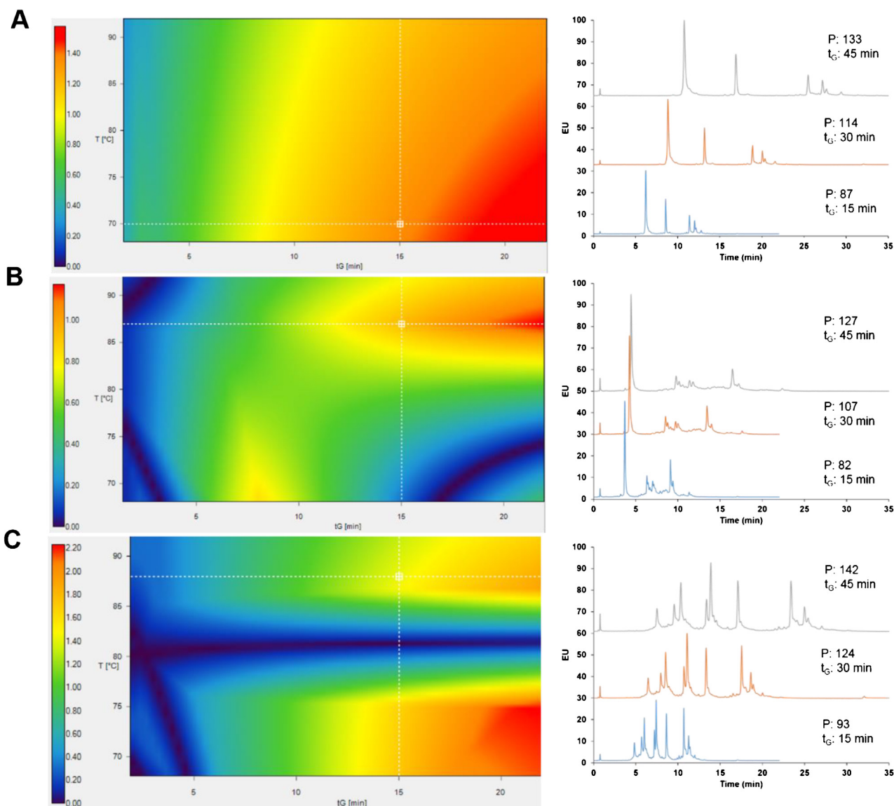
Fig. 5. Resolution maps and peak capacities at different gradient times of (A) NISTmAb, (B) cetuximab and (C) brentuximab vedotin using optimized gradient conditions described in Section 3.4.
