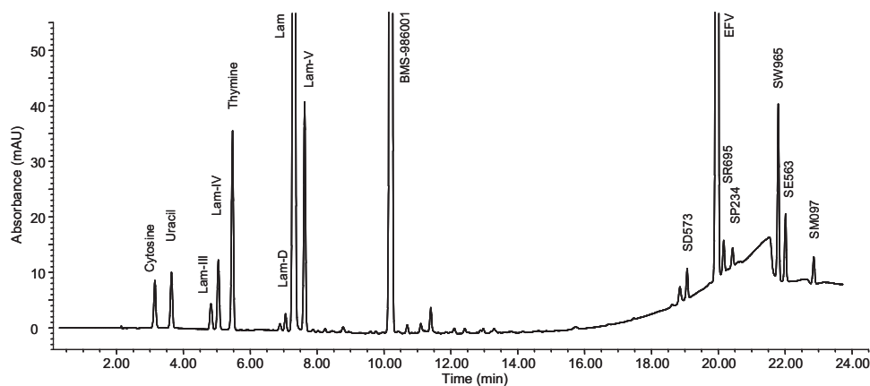
Fig. 2. RPLC separation of components in Lam/BMS-986001/EFV and related impurities/degradation products marker solution (marker solution A). Column: Discovery HS F5, 4.6 mm \times 150 mm, 3 \mu m, mobile phase A: 10 mM ammonium acetate, pH 5.5; mobile phase B: methanol; flow rate: 0.8 mL/min; column temperature: 35 ^{\circ} C; linear gradient: 5% B 0–0.7 min, 5–95% B 0.7–20.5 min, 95% B 20.5–23.8 min, 95–5% B 23.8–25.1 min, 95% B 25.1–30.4 min; UV detection: 260 nm; injection volume: 3.5 \mu L.
