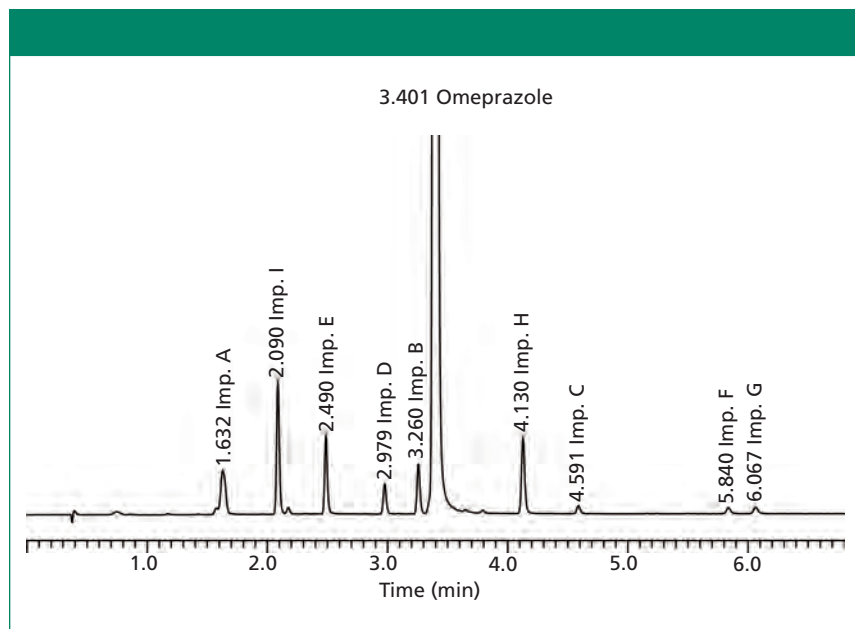
Figure 11: Experimental HPLC chromatogram of omeprazole spiked with its related impurities A–I for conditions after the transfer to the HPLC system (for details see text).
