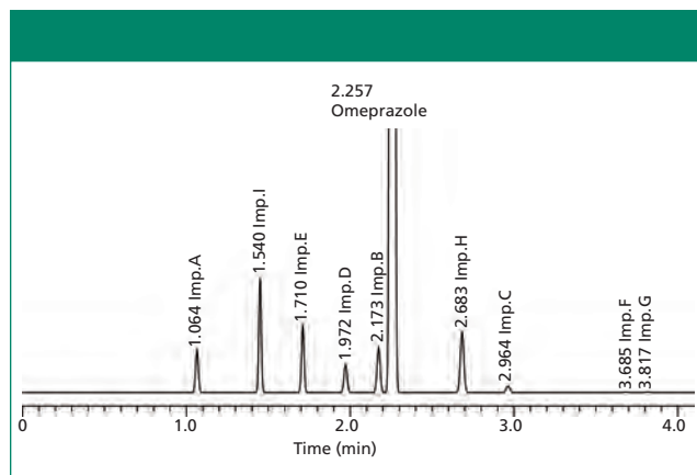
Figure 6: Predicted UHPLC chromatogram for omeprazole and its related impurities for conditions at the working point (for details see text).
