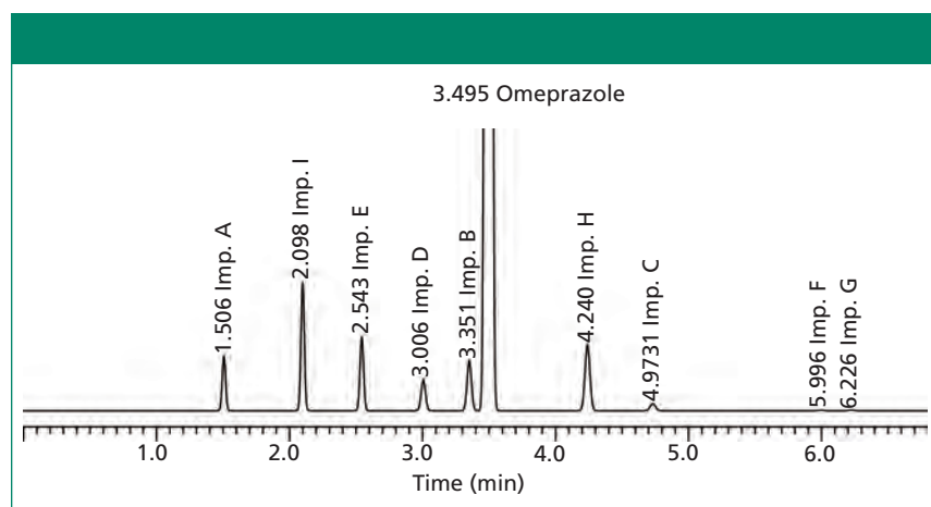
Figure 10: Predicted HPLC chromatogram for omeprazole and its related impurities for conditions after the transfer to the HPLC system (for details see text).
