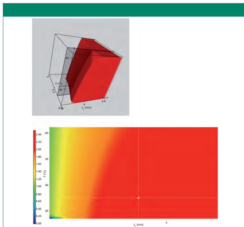
Figure 5: Three-dimensional resolution cube ( t_R/T/pH model) and the corresponding two-dimensional resolution map ( t_R/T model) at pH 8.75 for acetonitrile as the organic solvent in the UHPLC gradient method. The large red regions in the resolution maps represent the design space, in which performance criteria are met.
