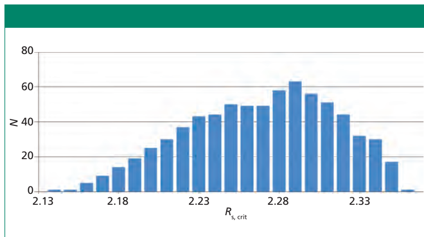
Figure 12: Frequency of the distribution of the resolution values R_{s,crit} for all 729 experiments of the robustness study after the transfer to the HPLC system. The six parameters t_G (7 min \pm 0.1 min), T (35 ^{\circ} C \pm 2 ^{\circ} C), pH (8.75 \pm 0.1), flow rate (1.9 mL/min \pm 0.1 mL/min), and the %B start (10% \pm 1%) and %B end (60% \pm 1%) of the gradient were varied at three levels (+1, 0, -1). All experiments still fulfill the requirement for resolution R_{s,crit} of no less than 2.0. That means that the failure is also 0.
