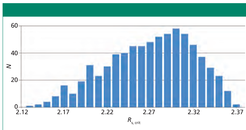
Figure 9: Frequency distribution of the R_{s,crit} values for all 729 experiments of the robustness study on the UHPLC system. The six parameters t_G (4 min \pm 0.1 min), T (35 °C \pm 2 °C), pH (8.75 \pm 0.1), flow rate (0.7 mL/min \pm 0.05 mL/min), and the %B start (10% \pm 1%) and %B end (60% \pm 1%) of the gradient were varied at three levels (+1, 0, -1). All experiments fulfill the requirement for resolution R_{s,crit} no less than 2.0. That means that the failure rate is 0, so there will be no method-related out-of-specification (OOS) results and production quality control will be smooth and robust.
