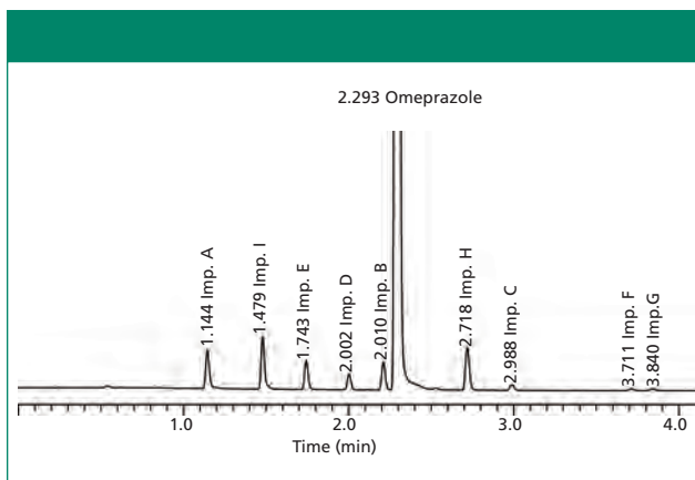
Figure 7: Experimental UHPLC chromatogram of omeprazole spiked with its related impurities A-I for conditions at the working point (for details see text).
