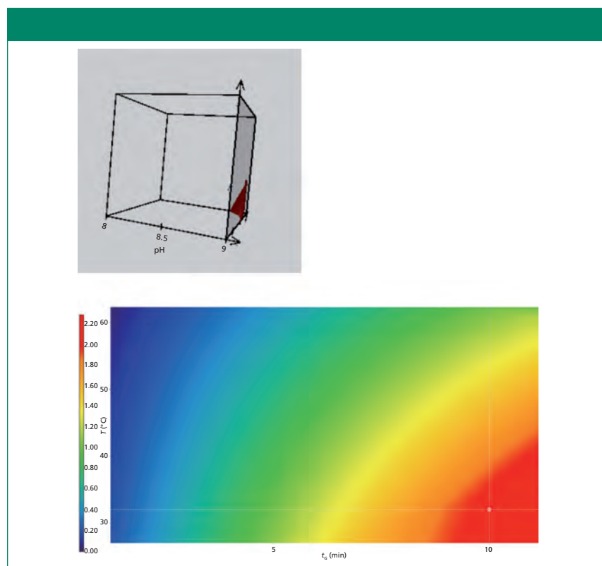
Figure 4: Three-dimensional resolution cube ( t_R/T/pH model) and the corresponding two-dimensional resolution map ( t_R/T model) at pH 9.0 for methanol as the organic solvent in the UHPLC gradient method. The red regions in the resolution maps represent the design space, in which the performance criteria are met.
