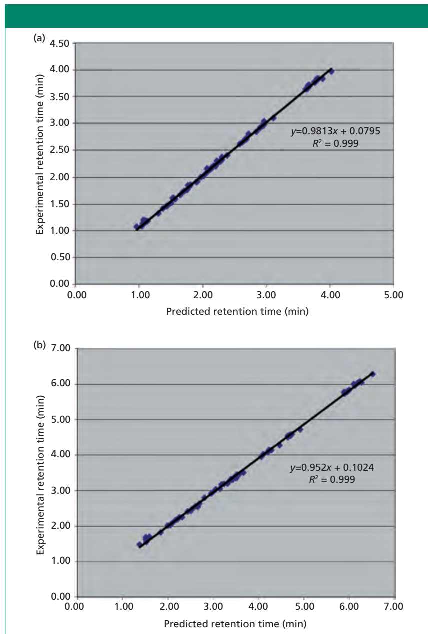
Figure 8: Plots of experimental retention time versus predicted retention time for (a) the UHPLC method and (b) after method transfer to HPLC.
